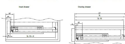
Installation dimensions
