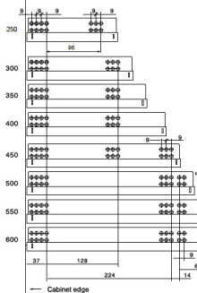
Hole pattern
