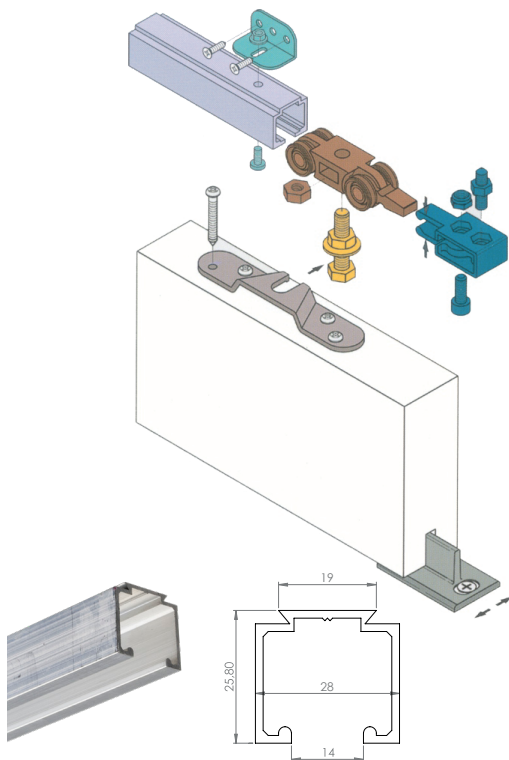
wall mounting steel clip
