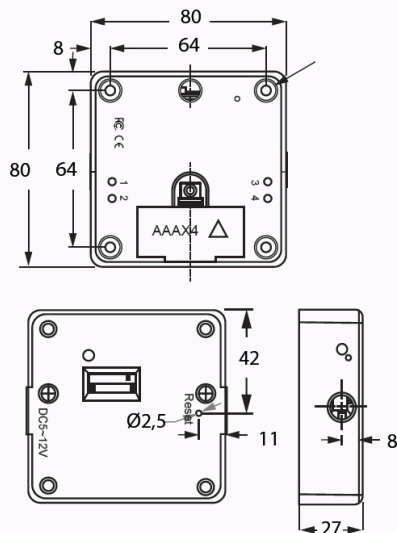
Lock body installation
