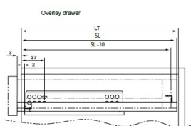
Installation dimensions
