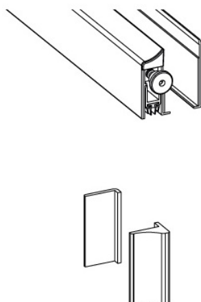
PLUNGER TYPE
