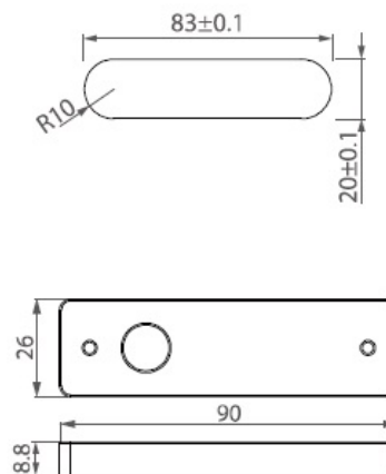
drilling template
