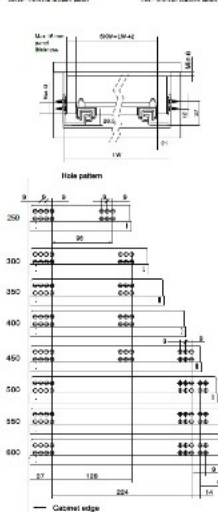
Installation dimensions
